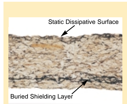
Microscopic cross section of PROTEKTIVE PAK's linerboard
