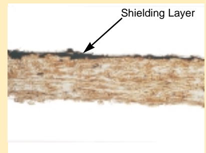
Microscopic cross section of carbon coated linerboard
