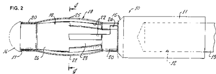
Redesigned Banana Plug Will Resist Abuse
