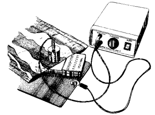
Shield Check Bag Tester
